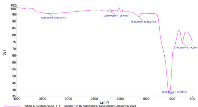
Figure 2. FTIR the silica synthesis curve from 4M pumice with purple color are almost similar
