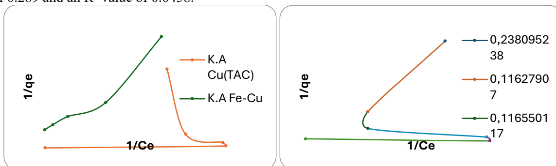
Gambar 2. Langmuir Isothermal Model for Cu(II) Adsorption by Activated Carbon, Activated Carbon-Cu(TAC) 2 , and Activated Carbon-Fe-Cu
