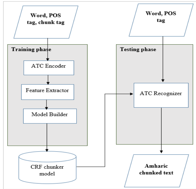
Figure 1. Architecture of CRFs based ATC
