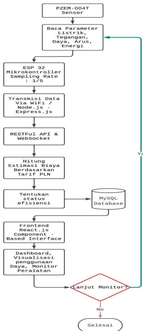
Gambar 1. Flowchart Sistem
