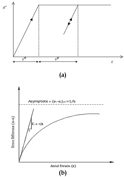
Gambar 9. Hubungan Tegangan-Regangan (A) Model Mohr Coulomb (Manual Plaxis) (B) Model Hardening Soil (Duncan & Chang, 1970)
