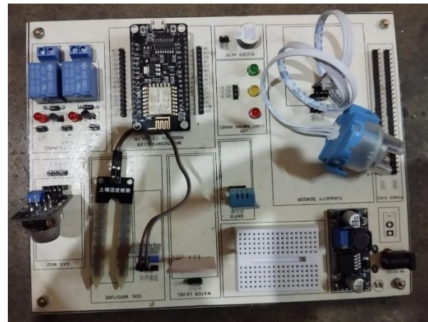
Gambar 2. Trainer sistem mikrokontroler NodeMCU ESP8266 V5 berbasis Internet of Things (IoT)
