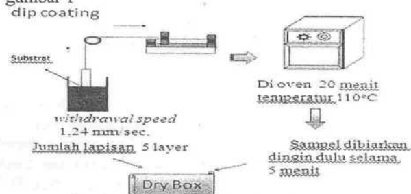
Gambar 1. Skema pelapisan ( coating )
