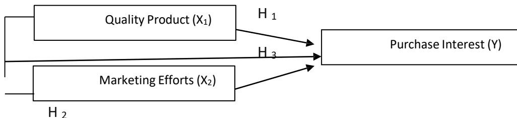
Figure 1. Framework Think
