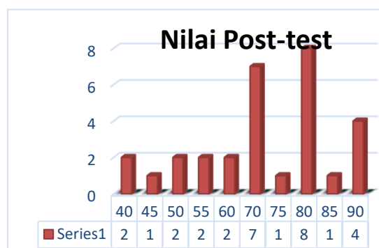
Gambar 1. Histogram Distribusi Frekuensi Post-test
