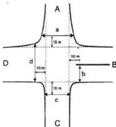
Gambar 3. Lebar pendekat rata-rata (MKJI, 1997).
